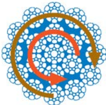
Rotation Resistant, 2 layer (11 to 13 outer strands)
